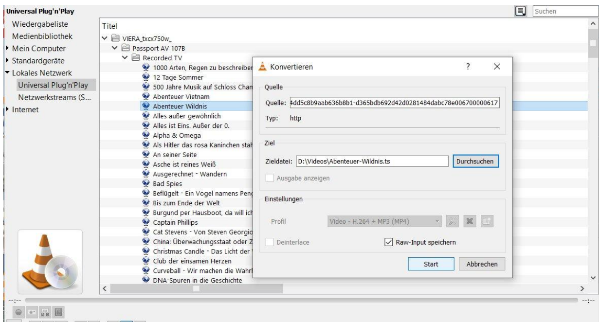
Fig. 2: VLC media player Version 2.0.7 Twoflower: The file shall be saved in raw modus as *.ts file (container)
