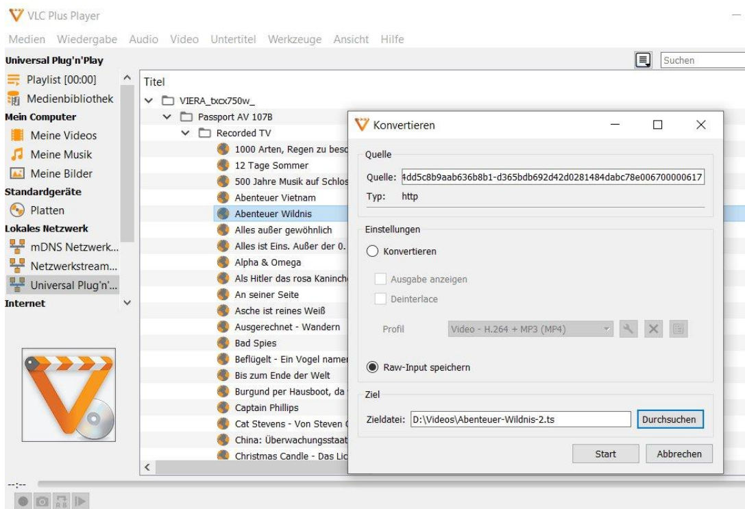
Fig. 5: VLC Plus Player Version 3.0.18 Vetinari: The file shall be saved in raw modus as *.ts file (container)
